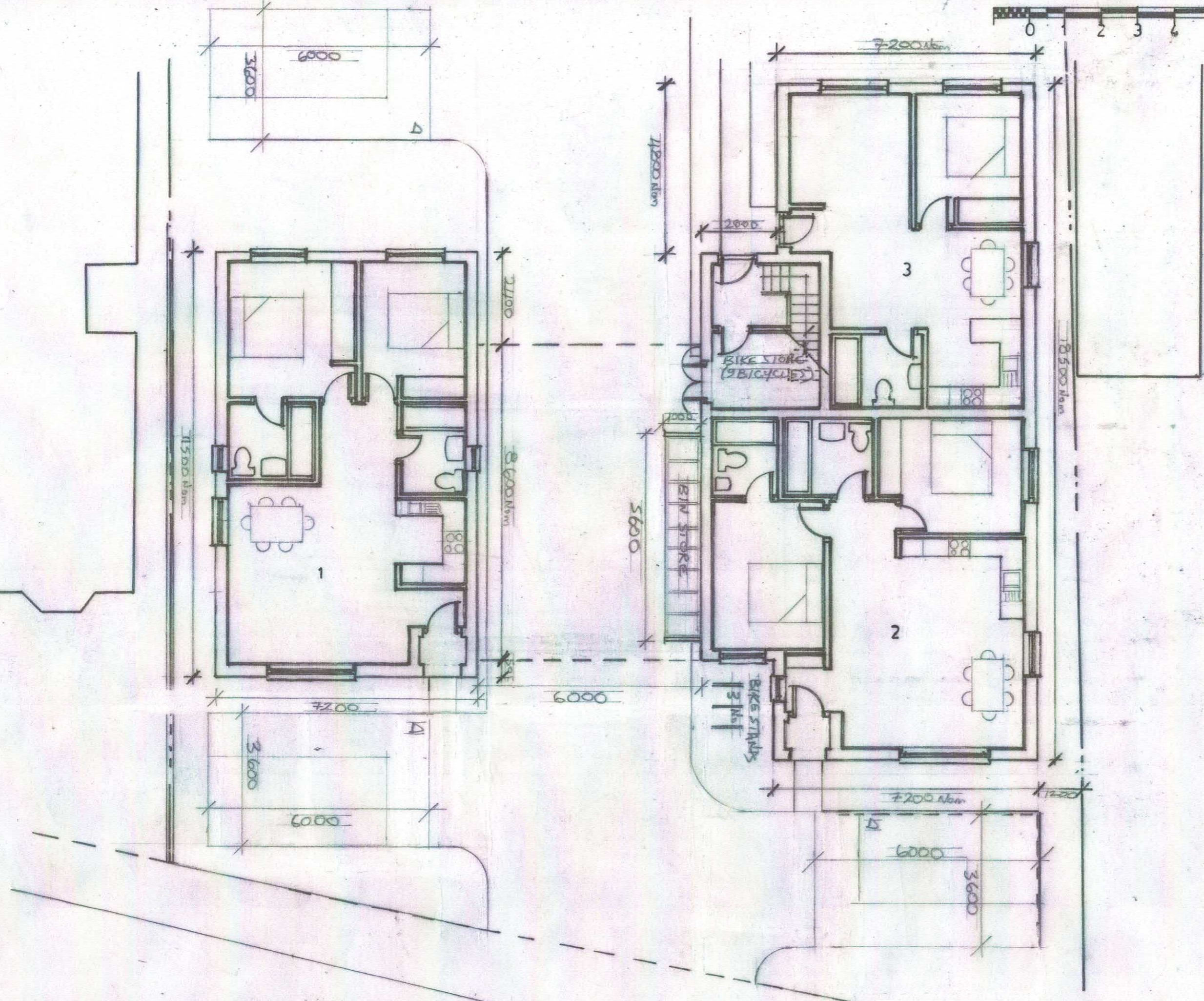
1 PROPOSED GROUND FLOOR PLAN 1:100 REVISED 11/9/20
