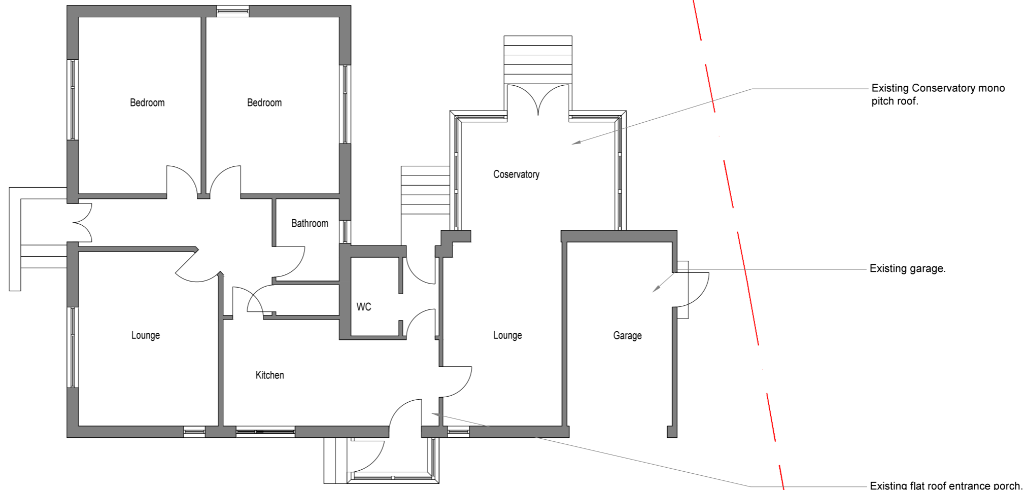
EXISTING ROOF PLAN 1:100
