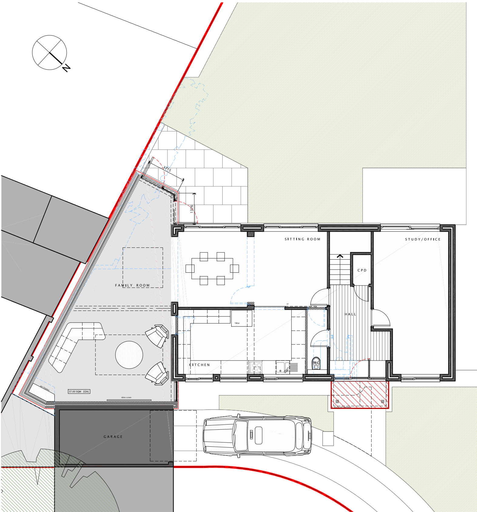
GROUND FLOOR PLAN PROPOSED 1:100
