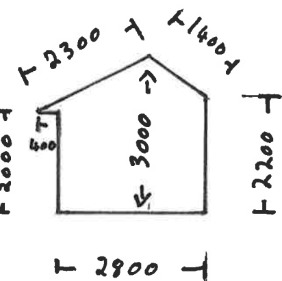
Side View from Road Side
