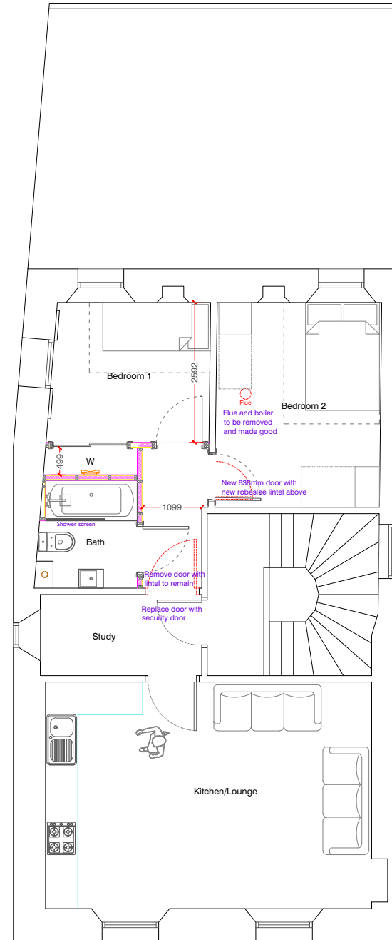
Proposed Second Floor Plan (scale 1:100)
