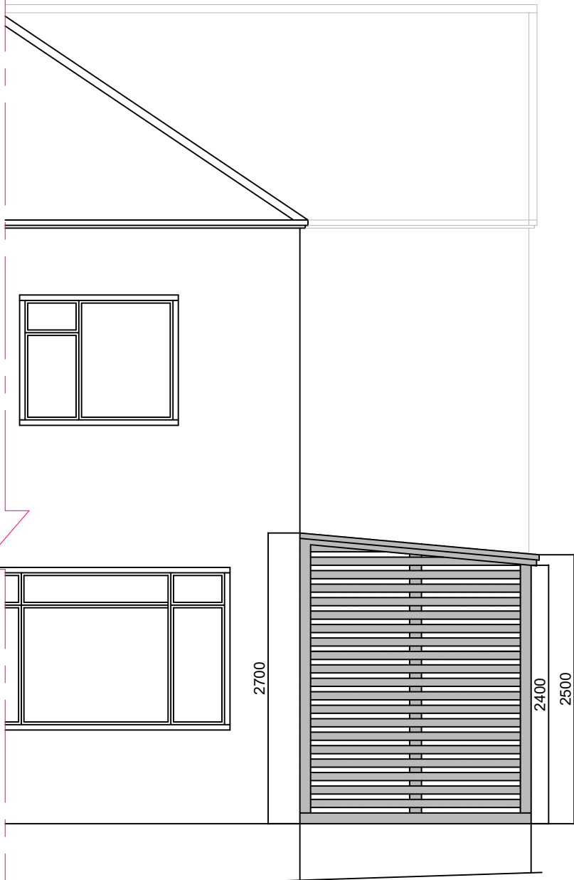
Proposed Part East Elevation
