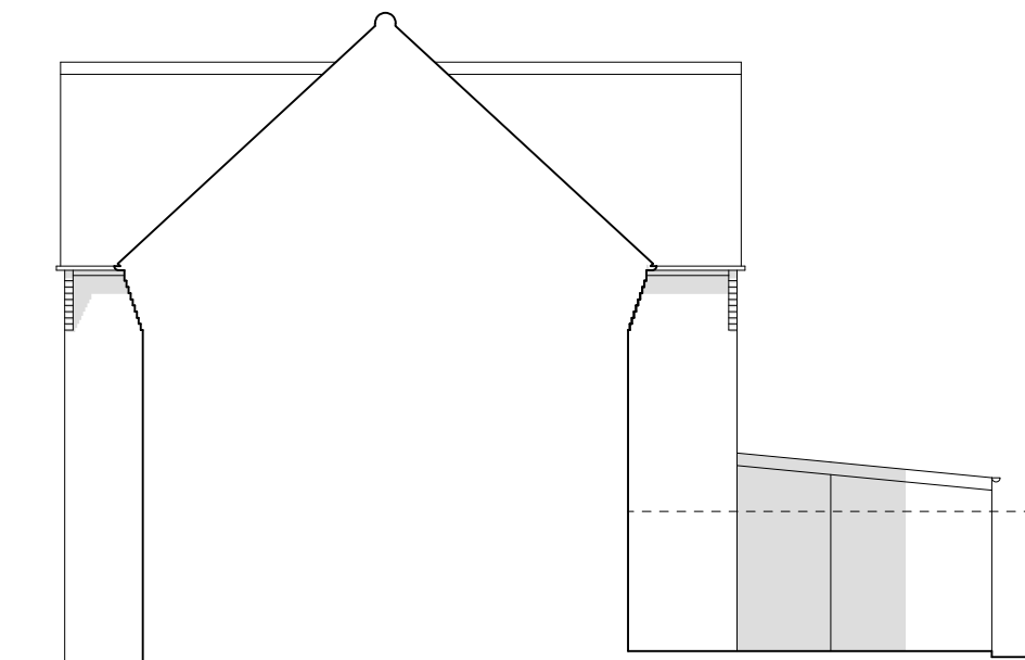
04 EXISTING SIDE (EAST) ELEVATION 1:100
