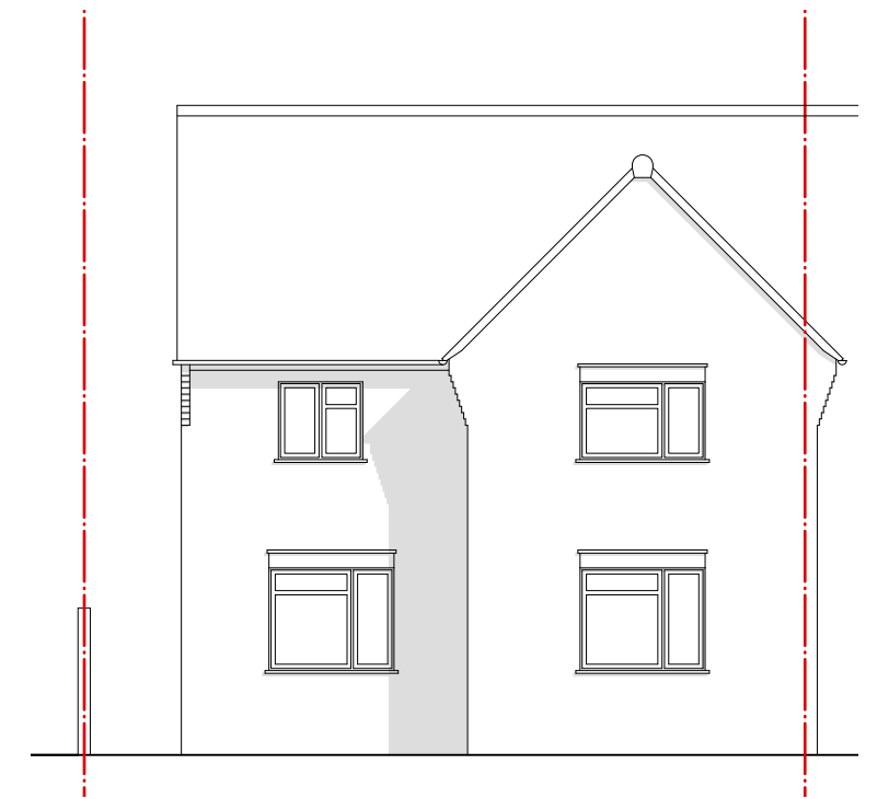
02 EXISTING FRONT ELEVATION 1:100
