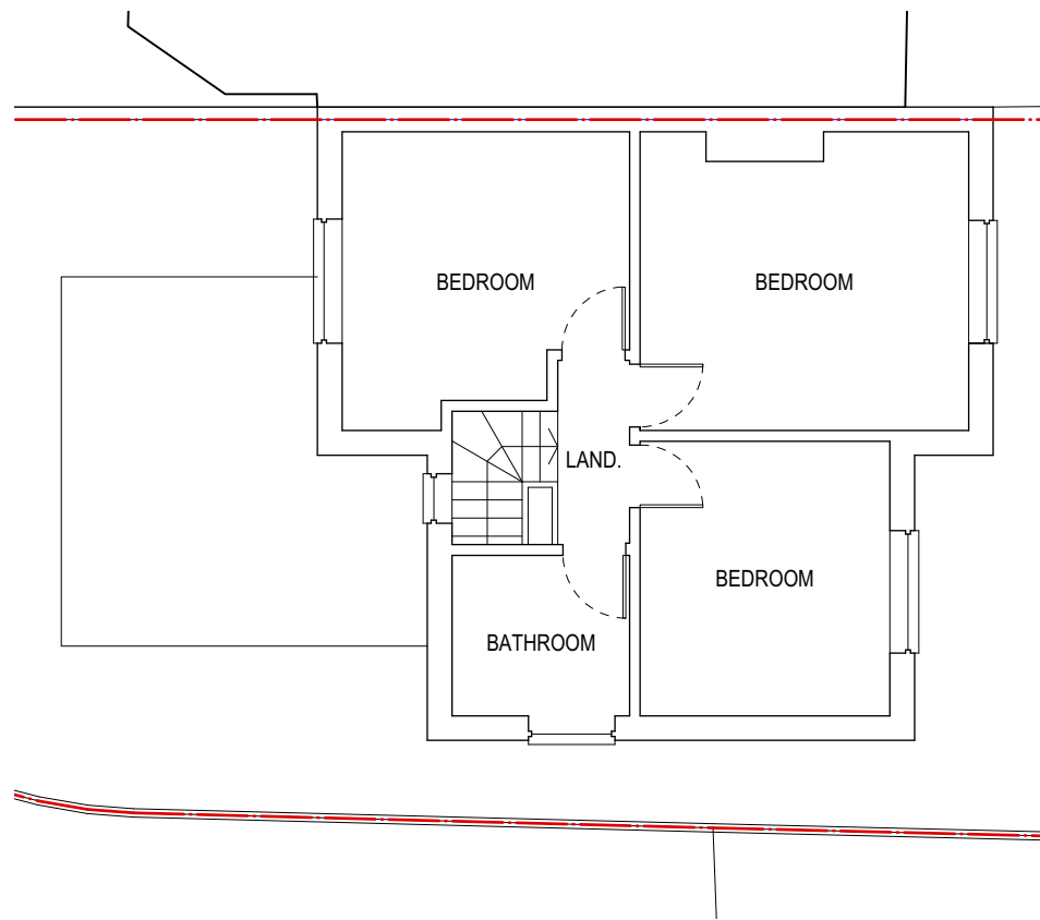
01 EXISTING FIRST FLOOR PLAN 1:100
