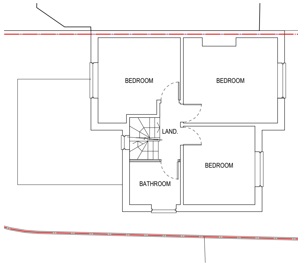
01 PROPOSED FIRST FLOOR PLAN 1:100
