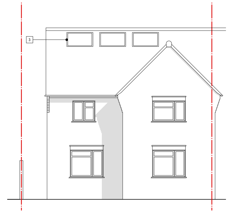
03 PROPOSED FRONT ELEVATION 1:100
