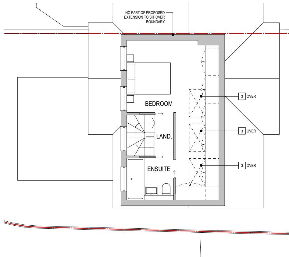
02 PROPOSED LOFT FLOOR PLAN 1:100
