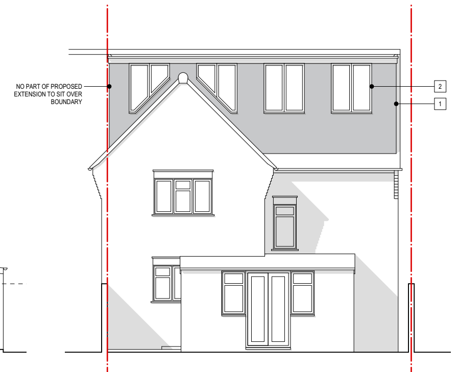
06 PROPOSED REAR ELEVATION 1:100
