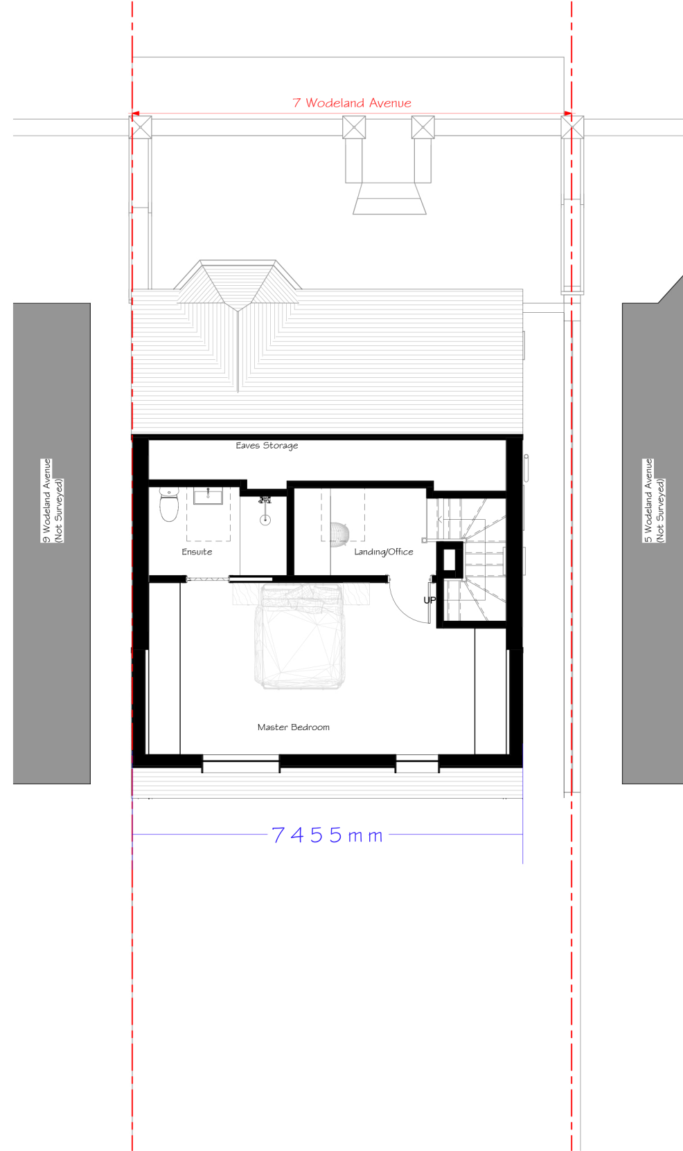
② Proposed Second Floor 1:100
