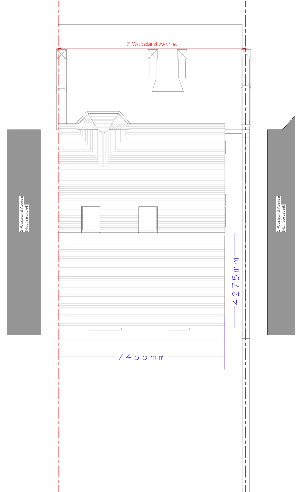
③ Proposed Roof 1:100
