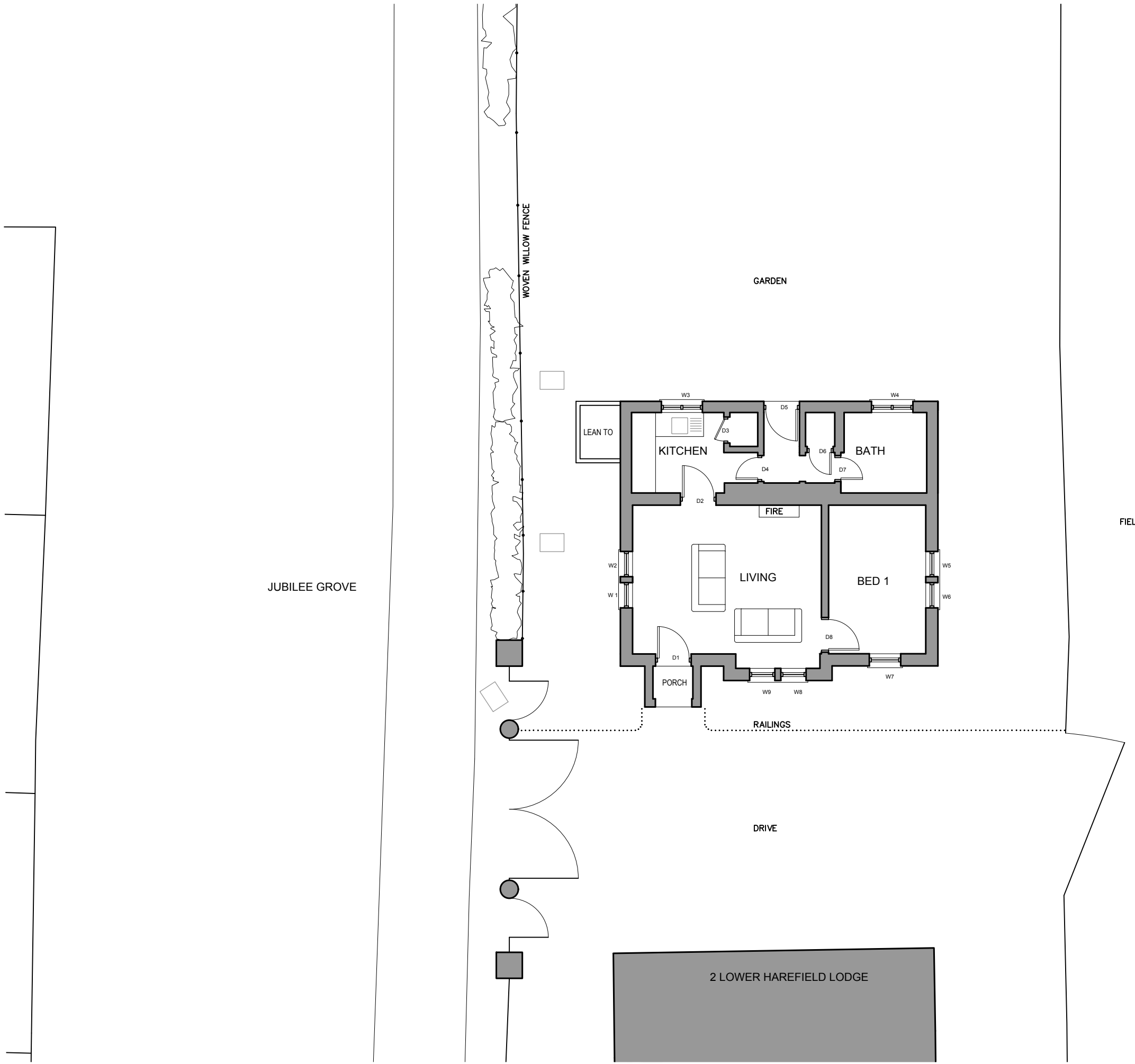
EXISTING GROUND FLOOR PLAN 1:100
