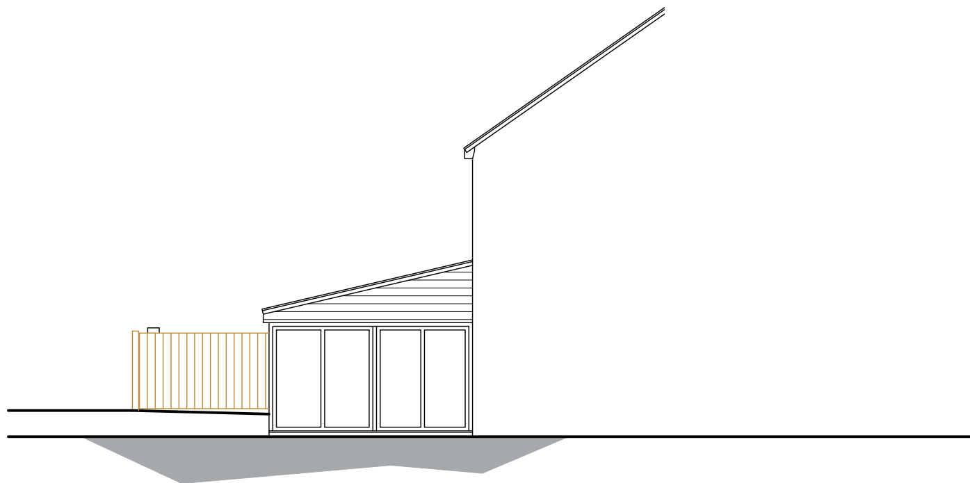
EAST ELEVATION 1:100
