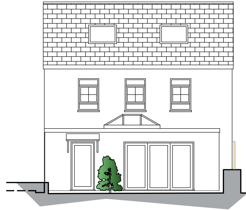
SOUTH ELEVATION 1:100
