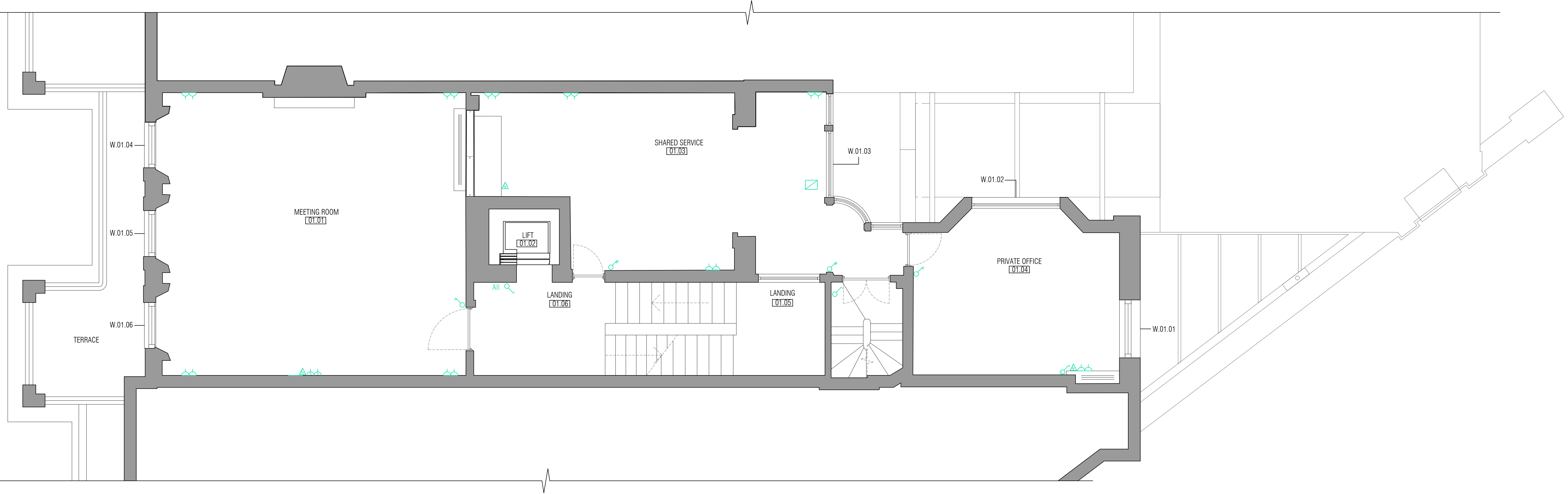
01.03.01 EXISTING FIRST FLOOR 2009 Scale 1:50@A1 - 1:100@A3
