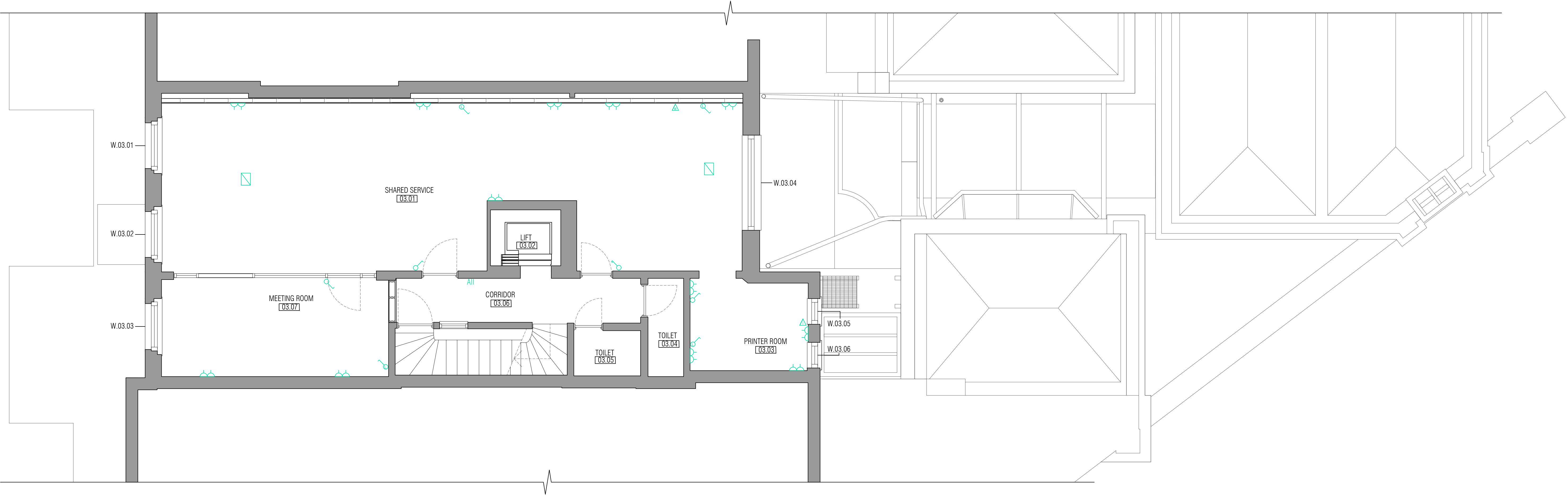
01.05.01 EXISTING THIRD FLOOR 2009 Scale 1:50@A1 - 1:100@A3
