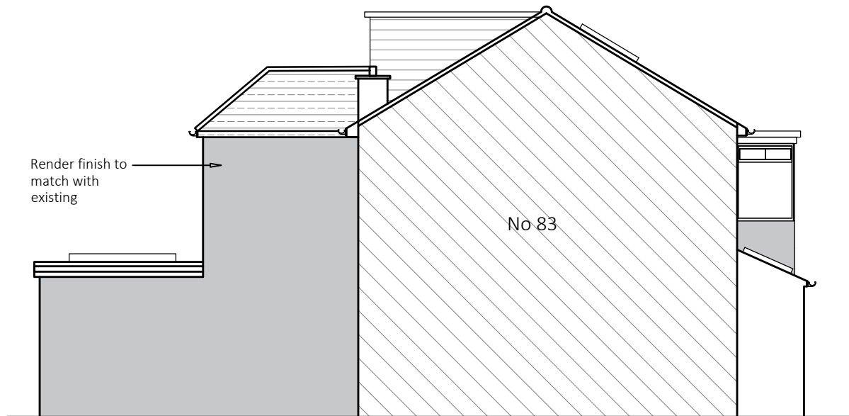
SIDE ELEVATION facing No 83
