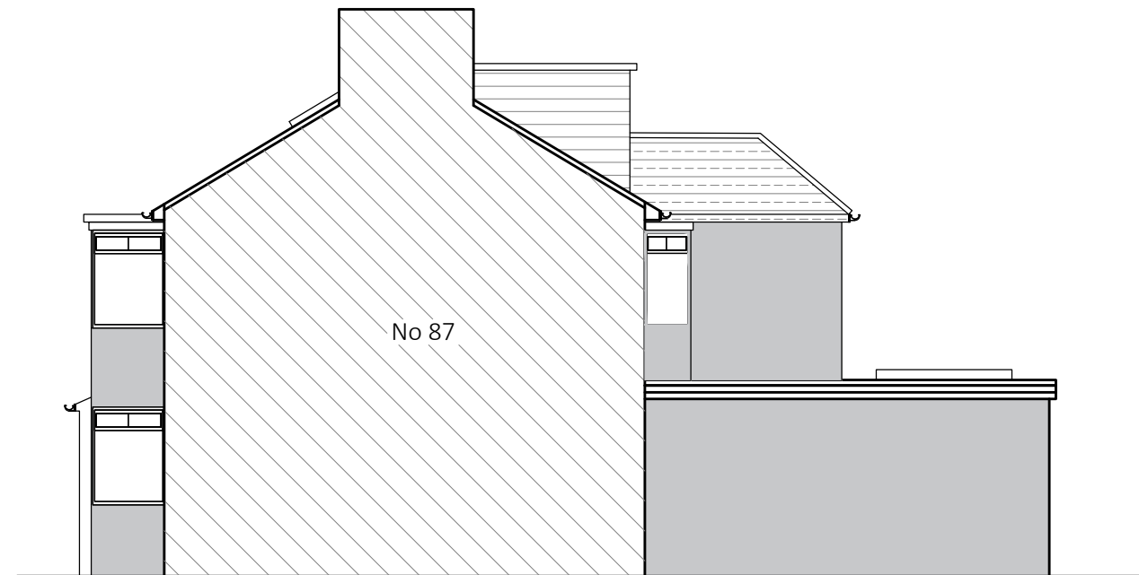
SIDE ELEVATION facing No 87
