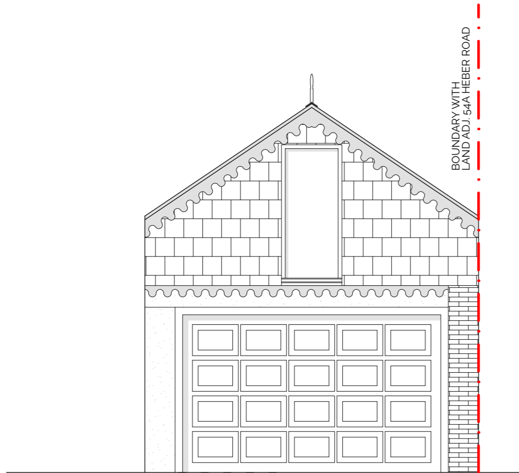
EXISTING FRONT ELEVATION 1:50
