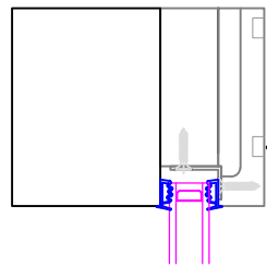
Direct Glazed Window Head Rail
