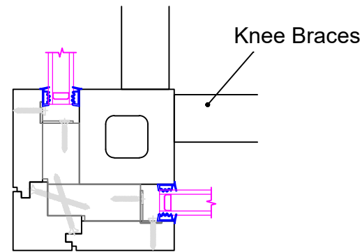
PLAN VIEW OF CORNER POST Scale 1:5
