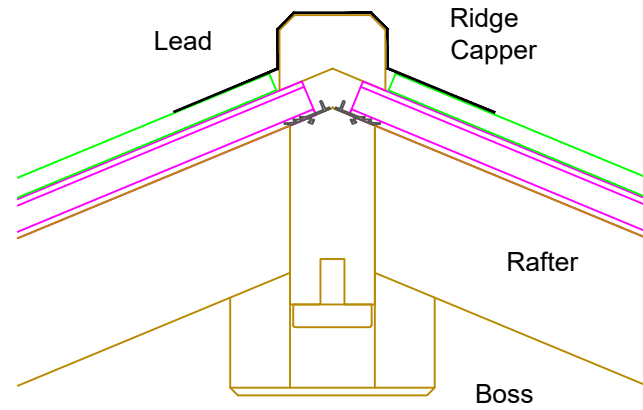
Ridge Detail
