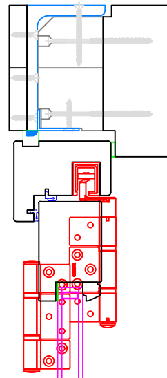
Door Head Rail
