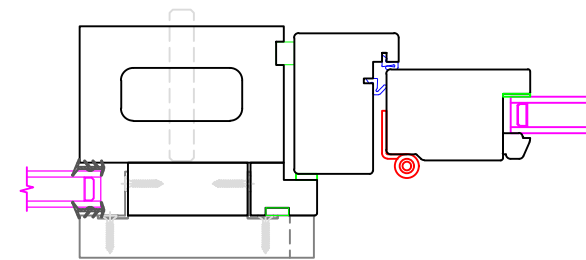
PLAN VIEW OF BI-FOLD DOORS Scale 1:5
