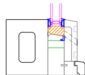
Direct Galzed Window Bottom Rail
