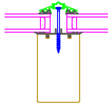
Rafter Detail
