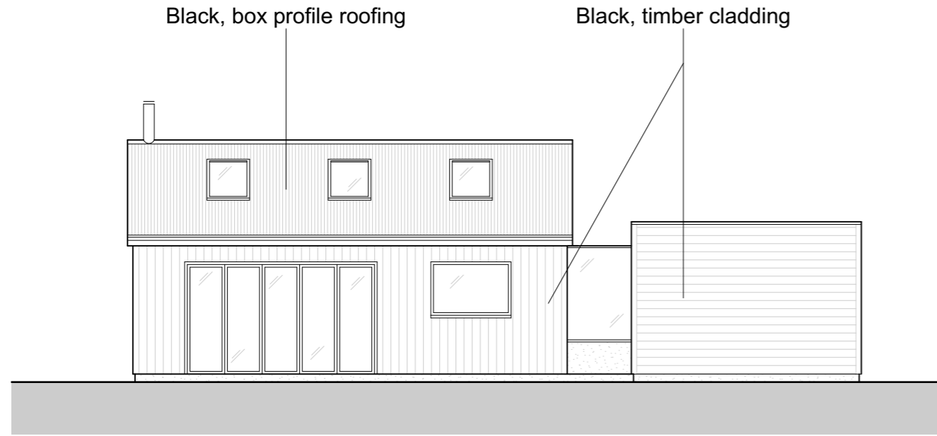
Proposed SW Elevation 1:100
