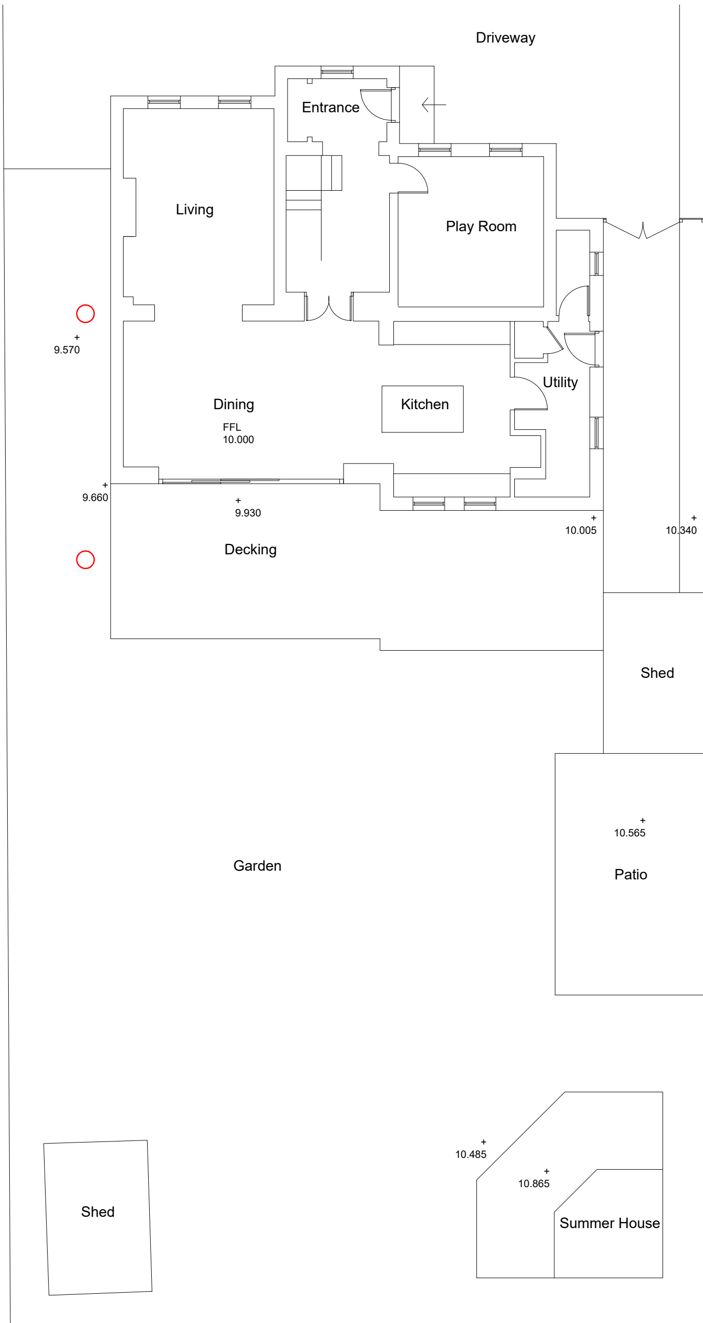
Existing Site Plan
