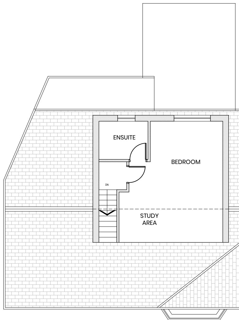
Proposed GA Loft Plan 1:100
