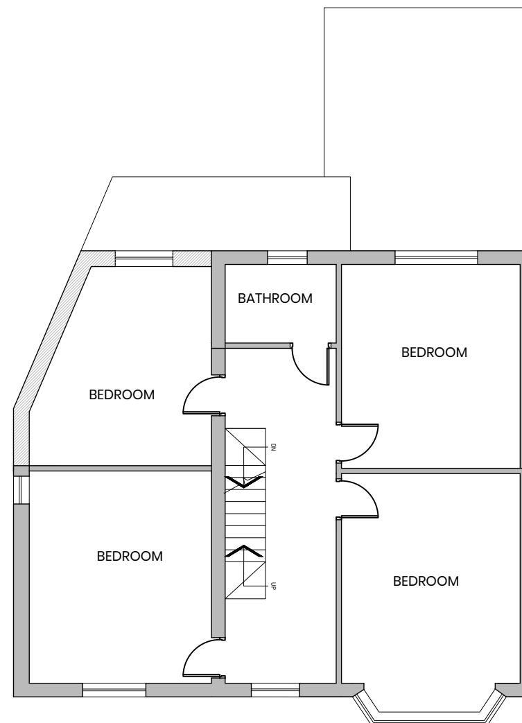
Proposed GA First Floor 1:100
