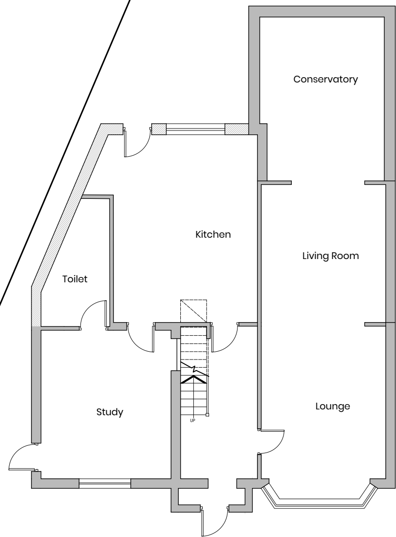
Proposed GA Ground Floor 1:100
