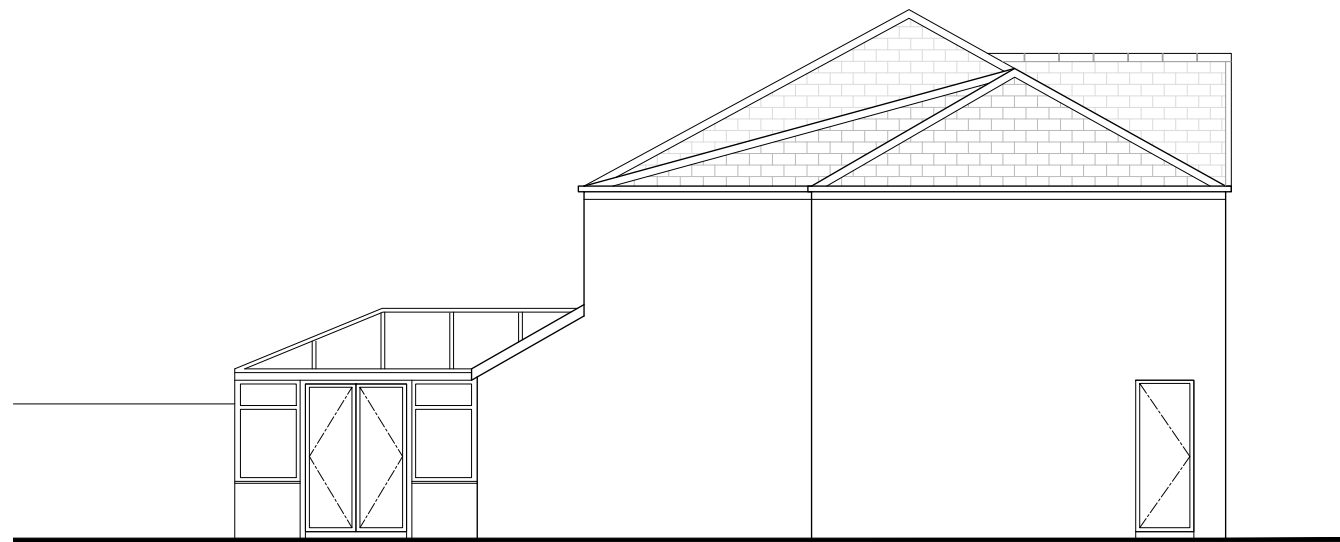
As Approved GA Side Elevation (NE) 1:100
