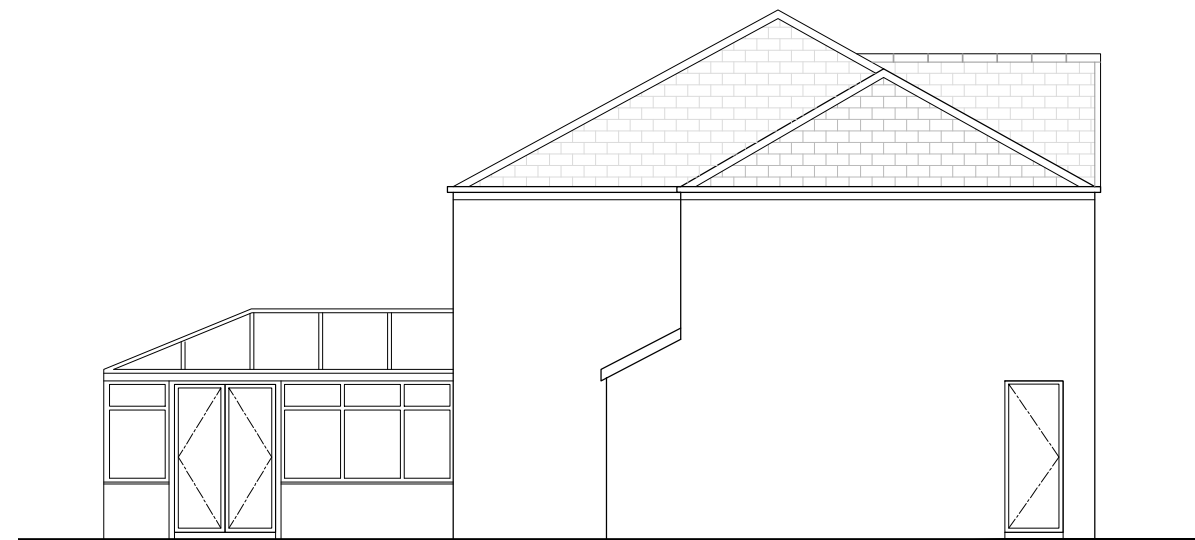
Existing GA Side Elevation (NE) 1:100
