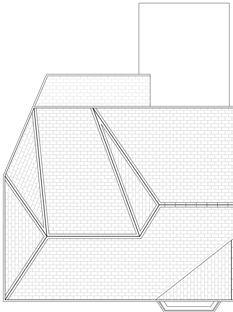
As Approved GA Roof Plan 1:100
