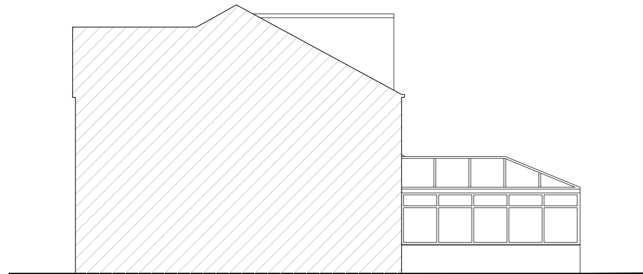
As Approved GA Side Elevation (SW) 1:100
