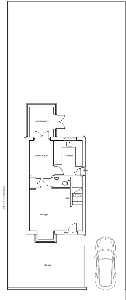
SITE PLAN
