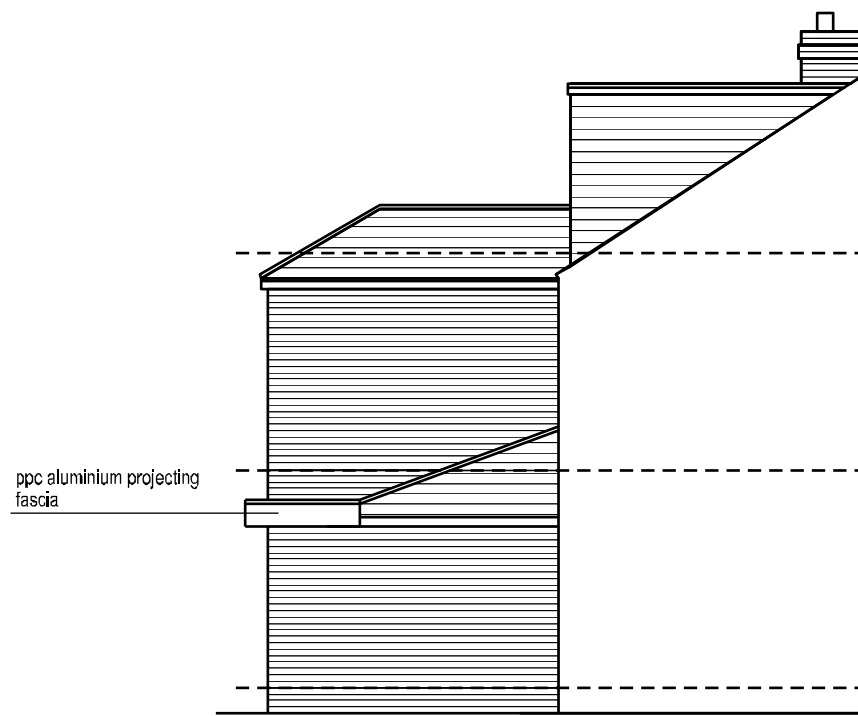
North Elevation
