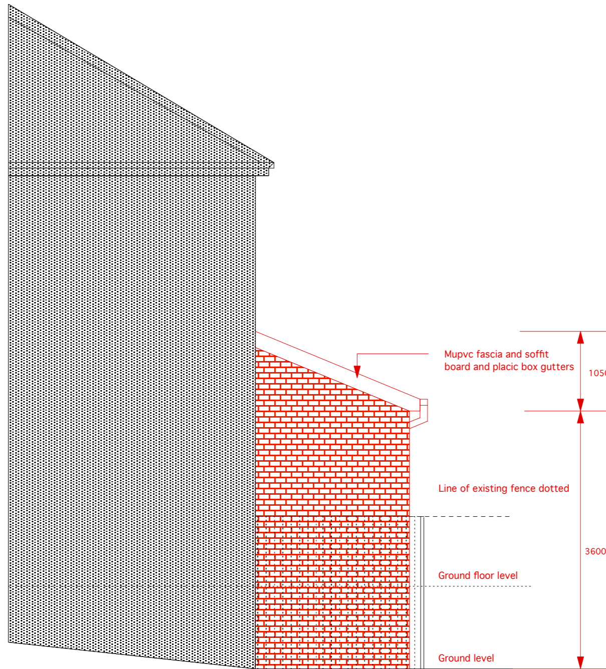
Side Elevation as Proposed as viewed from adjoining property
