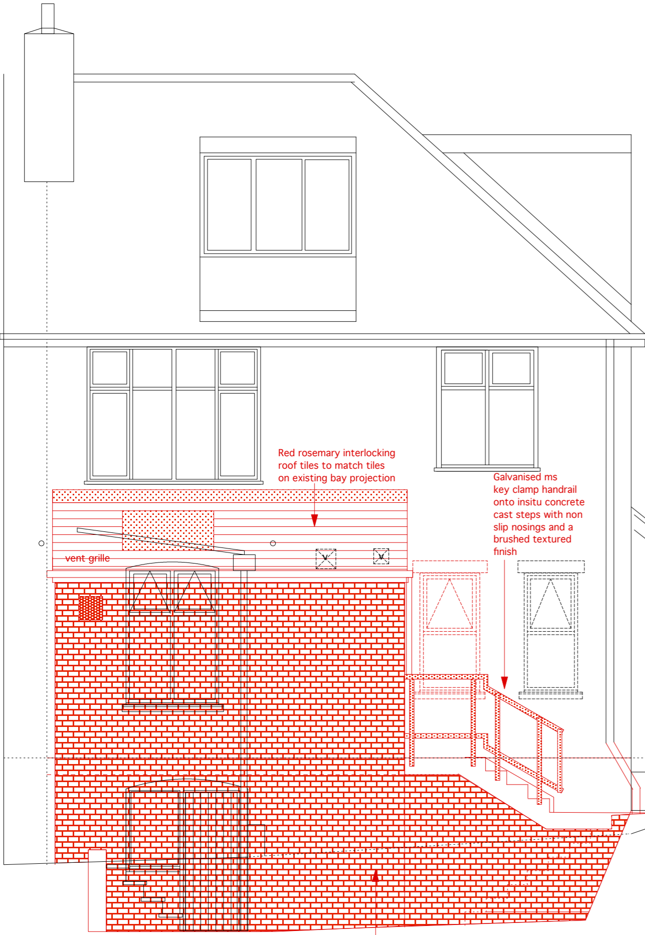
Rear Elevation as Proposed
