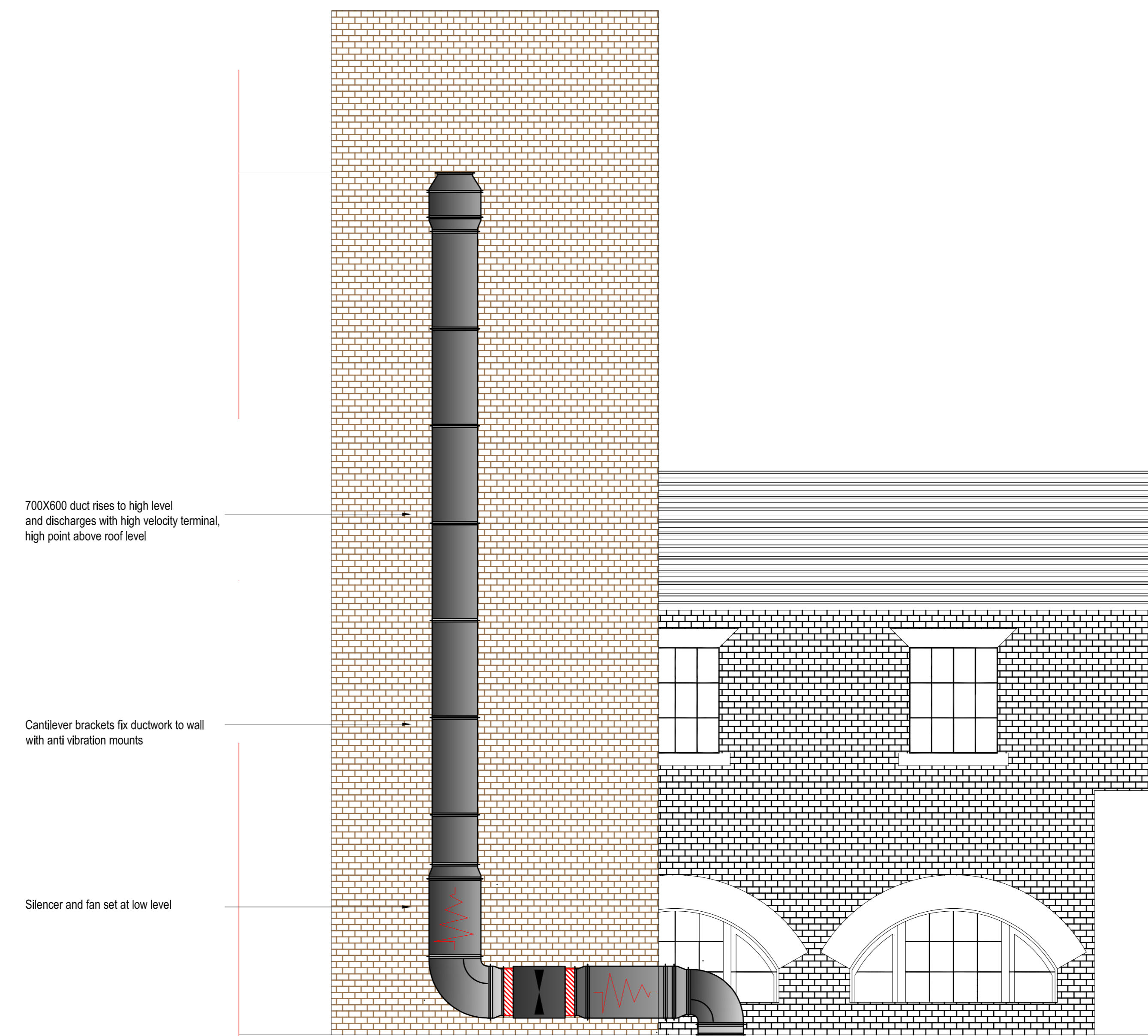
Internal elevation from plant deck roof AA Exhaust duct
