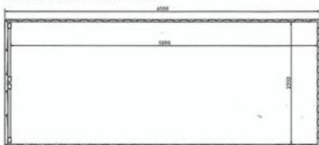
20ft Shipping Container - Plan
