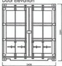
20ft Shipping Container - Door Elevation
