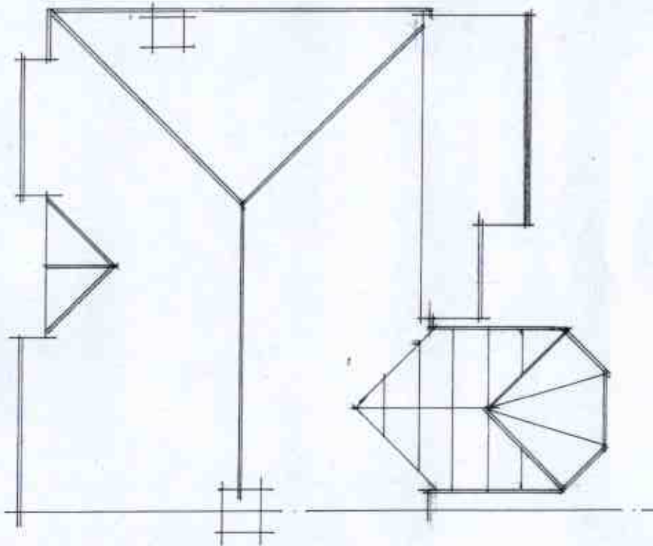
Existing roof 1:100
