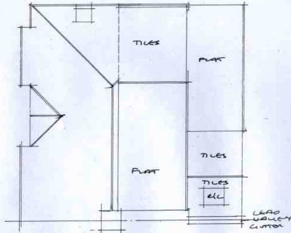
Proposed roof 1:100
