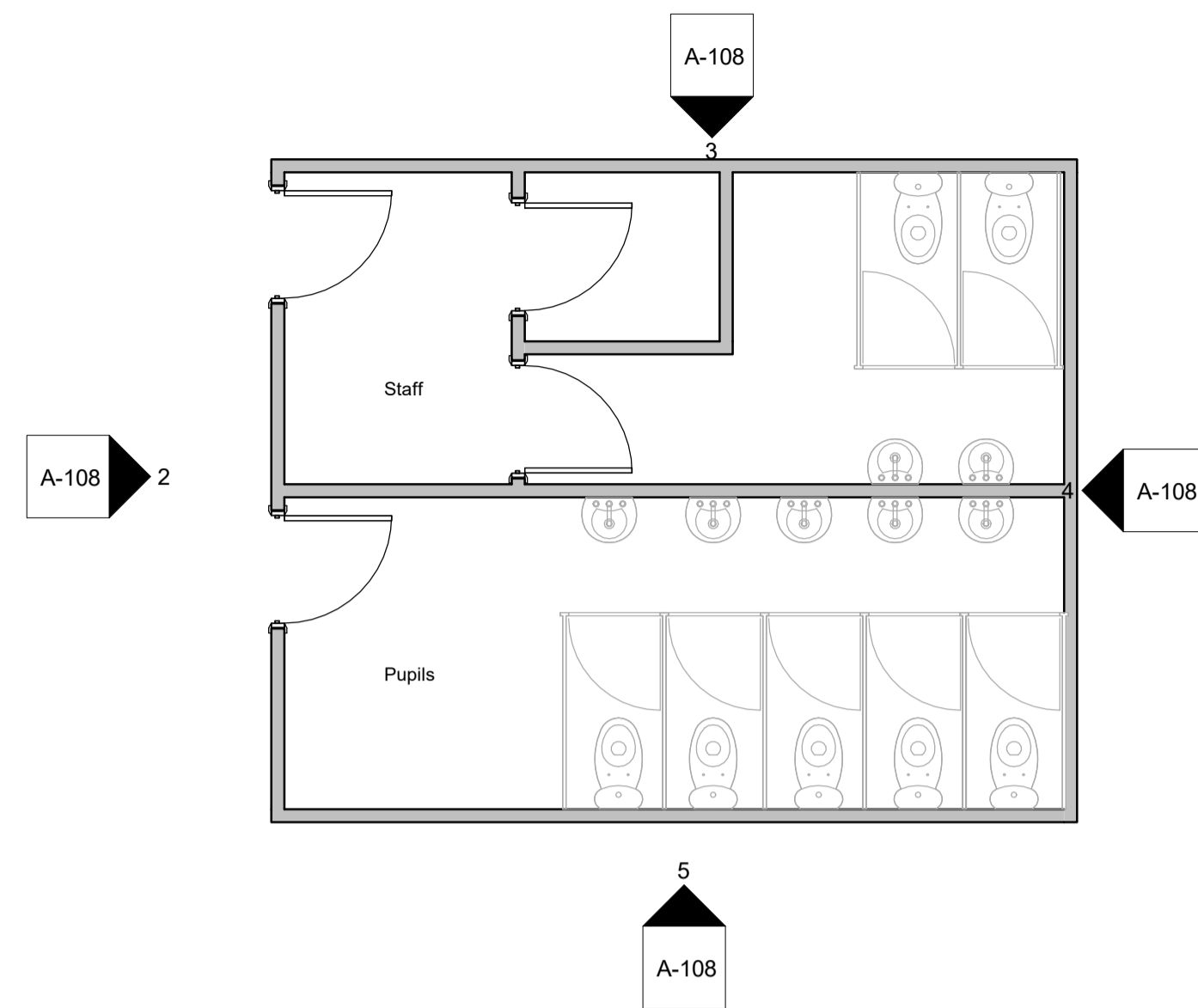
Temp Toliet Block Plan 1 : 50
