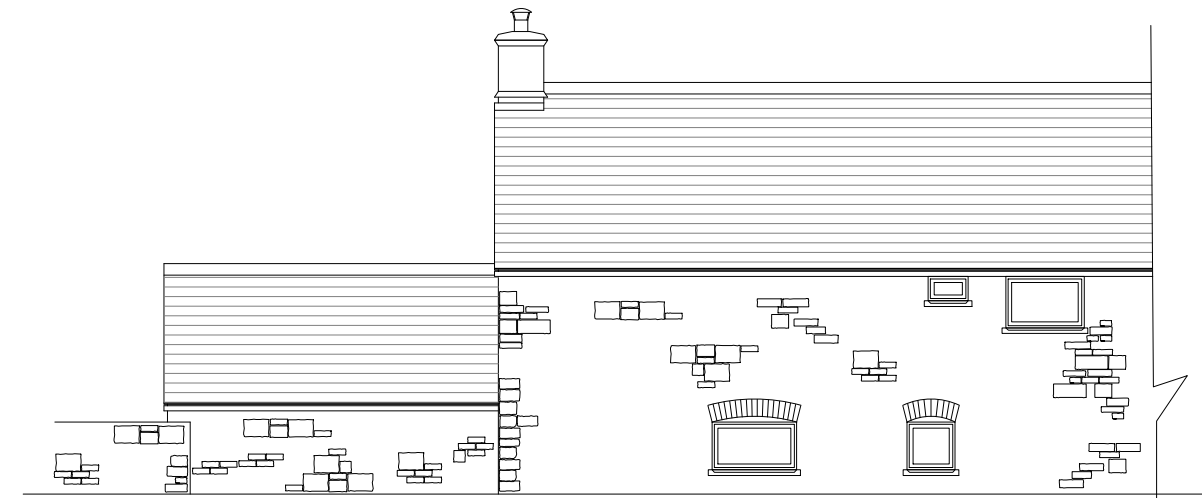
REAR ELEVATION 1:100
