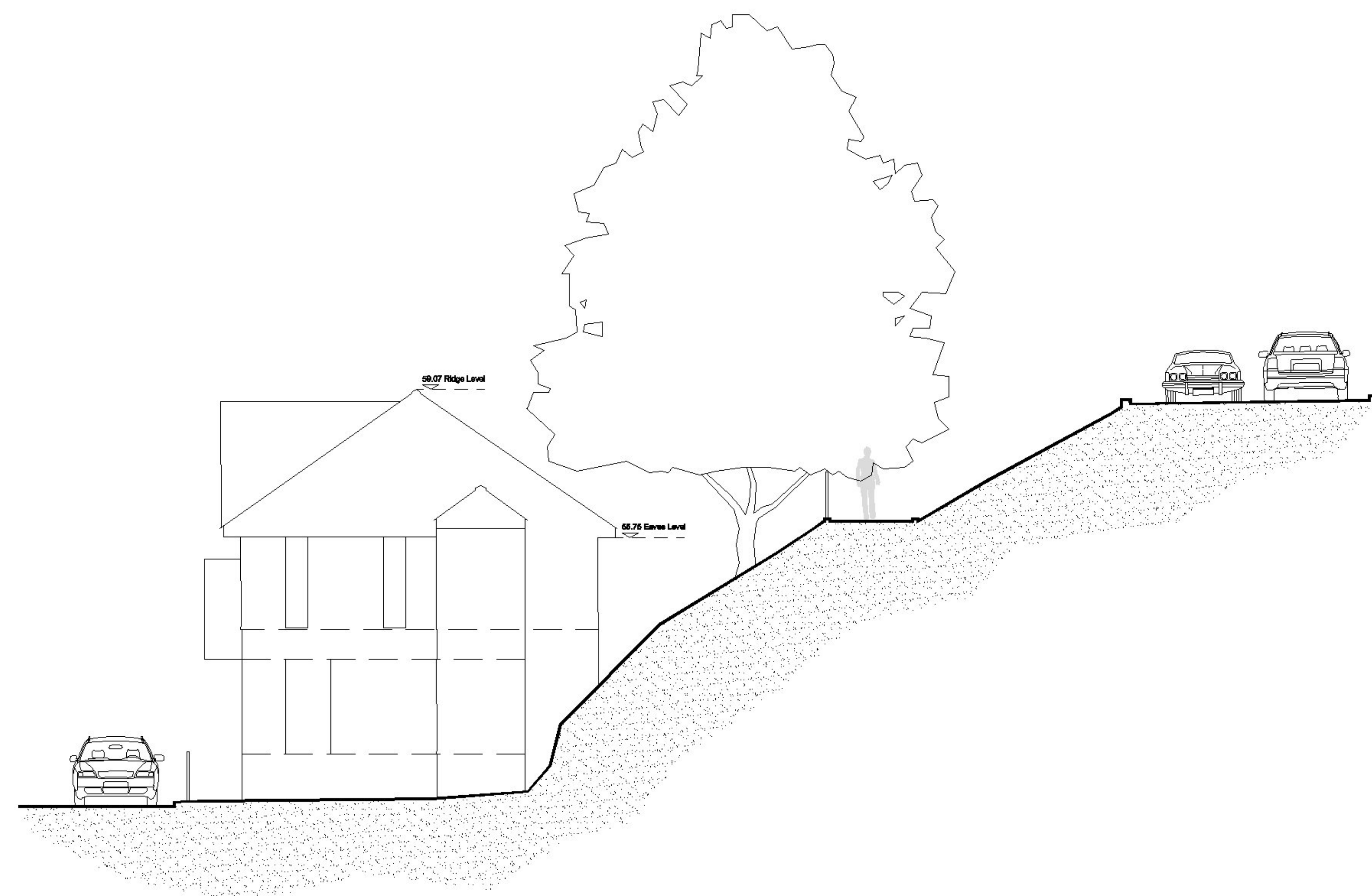
Site Longitudinal Section towards East 1:100
