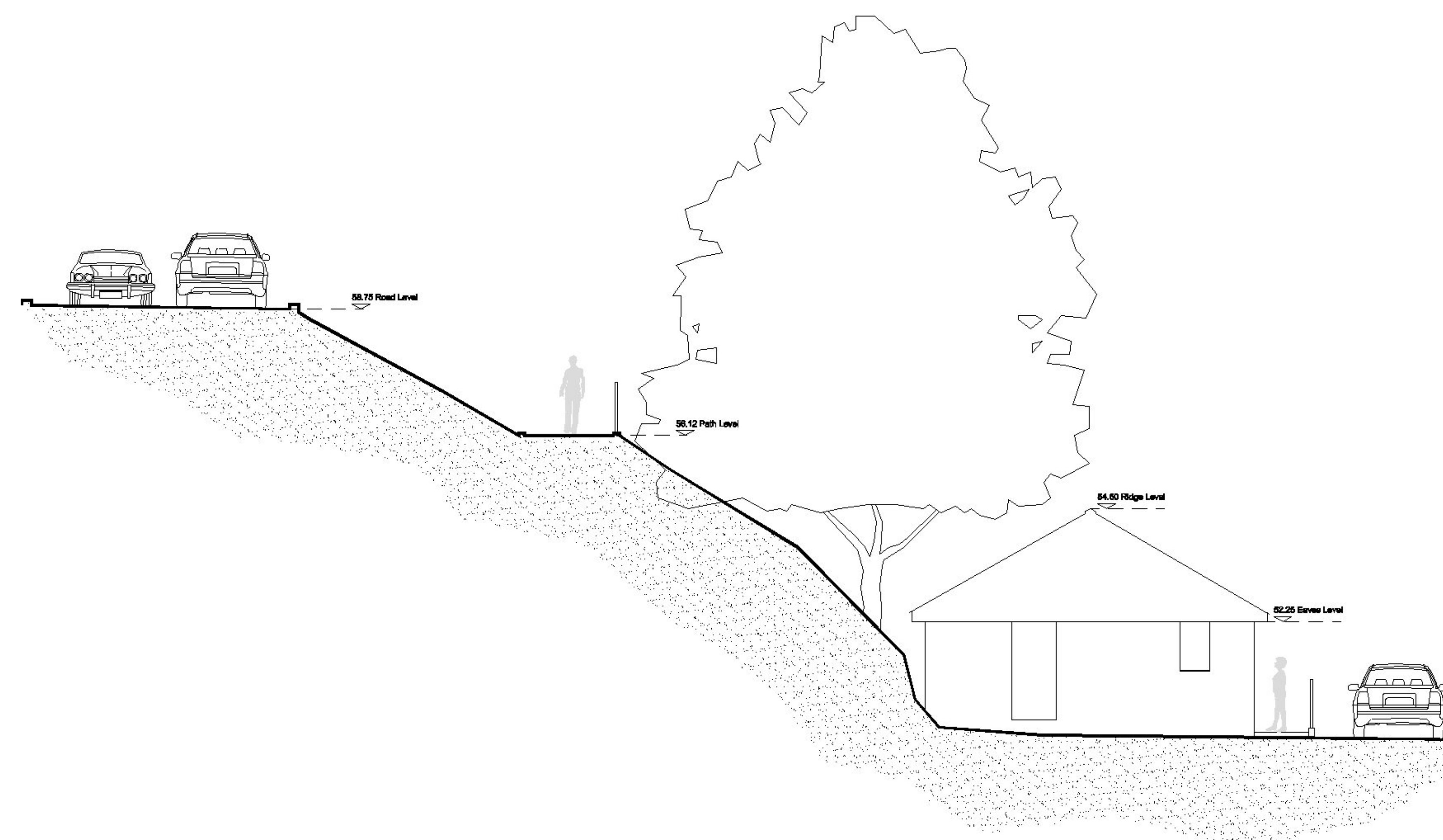
Site Longitudinal Section towards West 1:100
