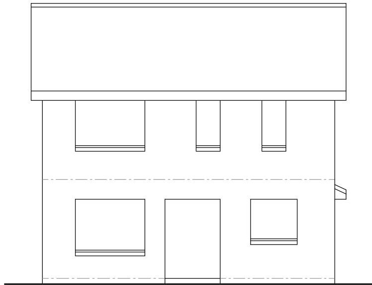
South-East Elevation
