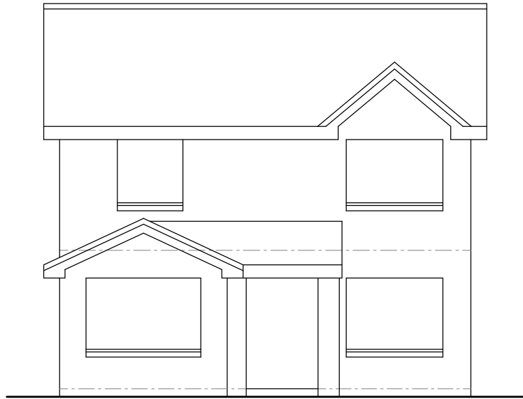
North-West Elevation
