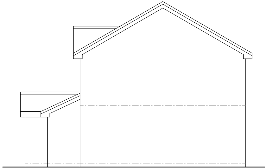
South-West Elevation
