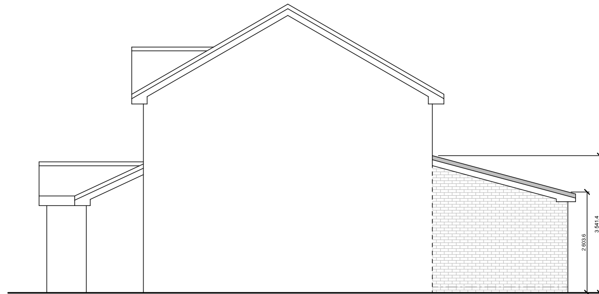
South-West Elevation
