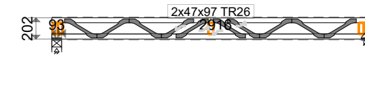
PS6- 1 no. 1-ply 11 kg
