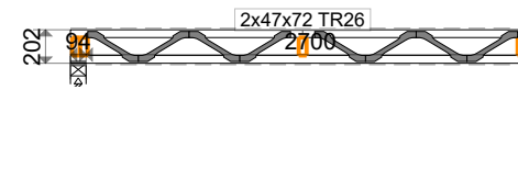
PS5G- 1 no. 2-ply 29 kg
