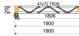
PS5G- 1 no. 2-ply 29 kg
