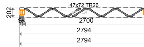
PS3- 5 no. 1-ply 11 kg
