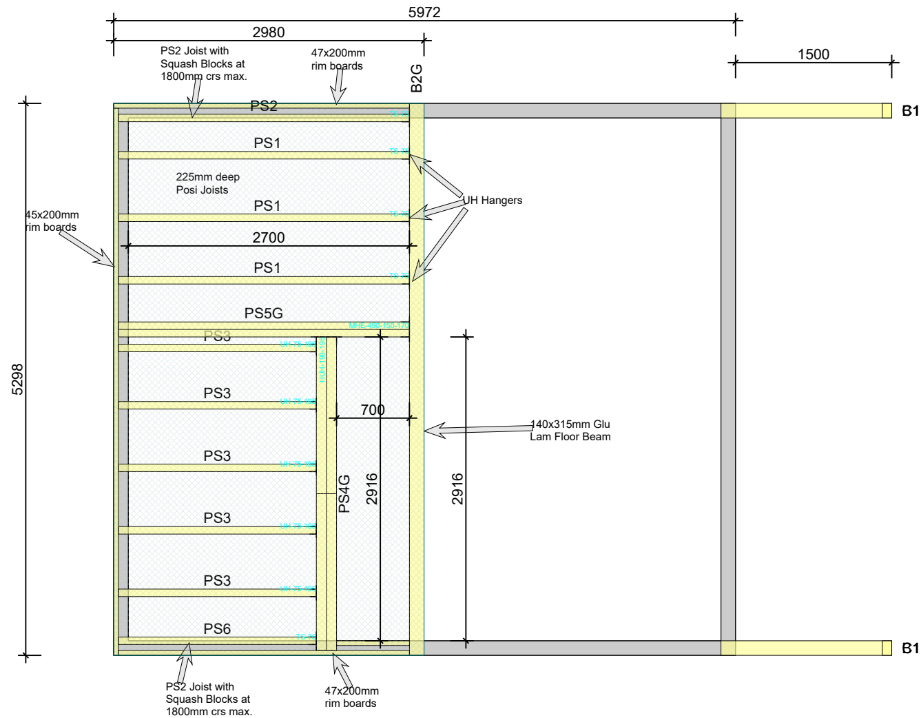
Mezzanine Floor in 202mm Posi Joists at 600mm crs max.
