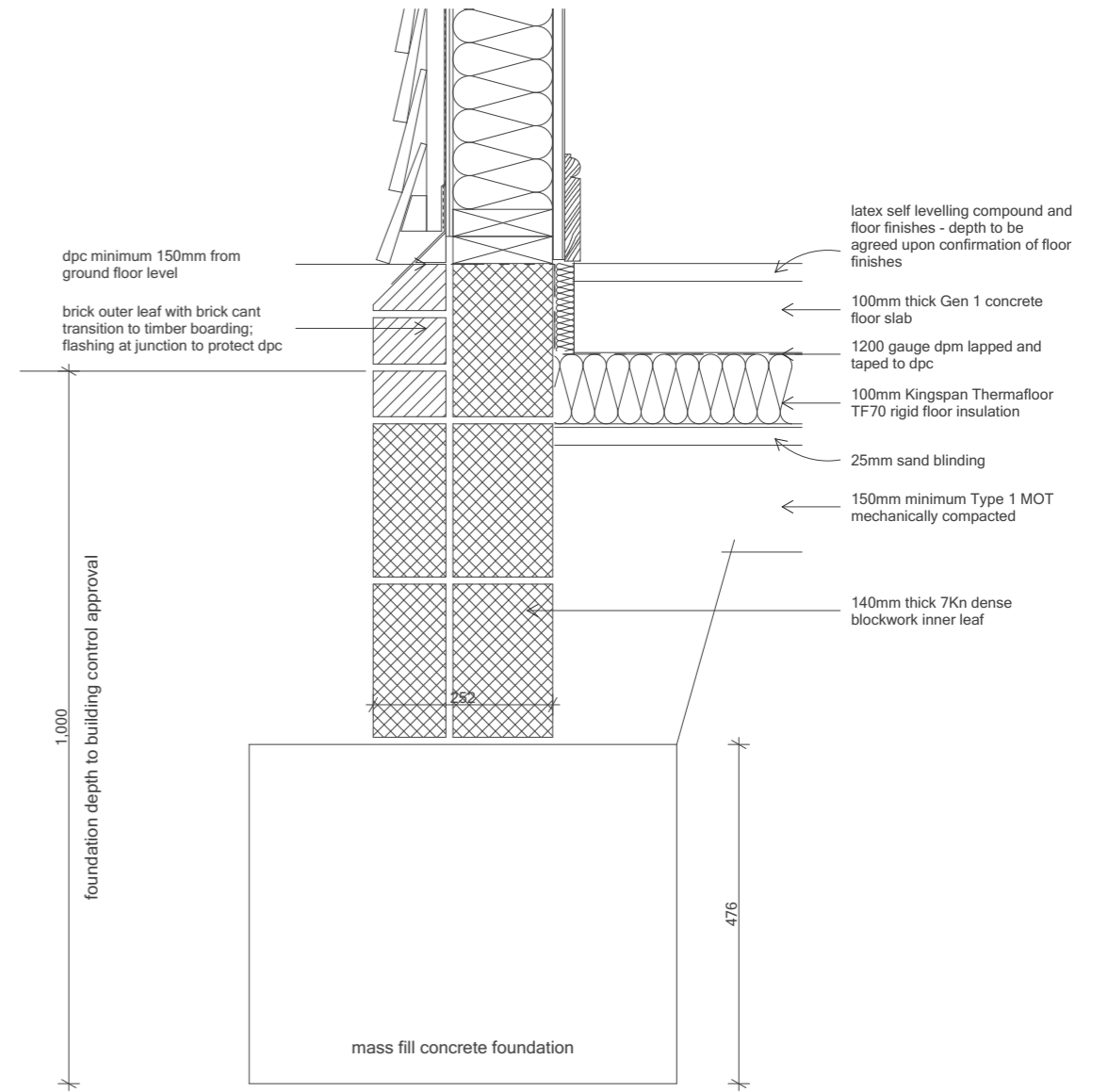
TYPICAL FOUNDATION DETAIL
