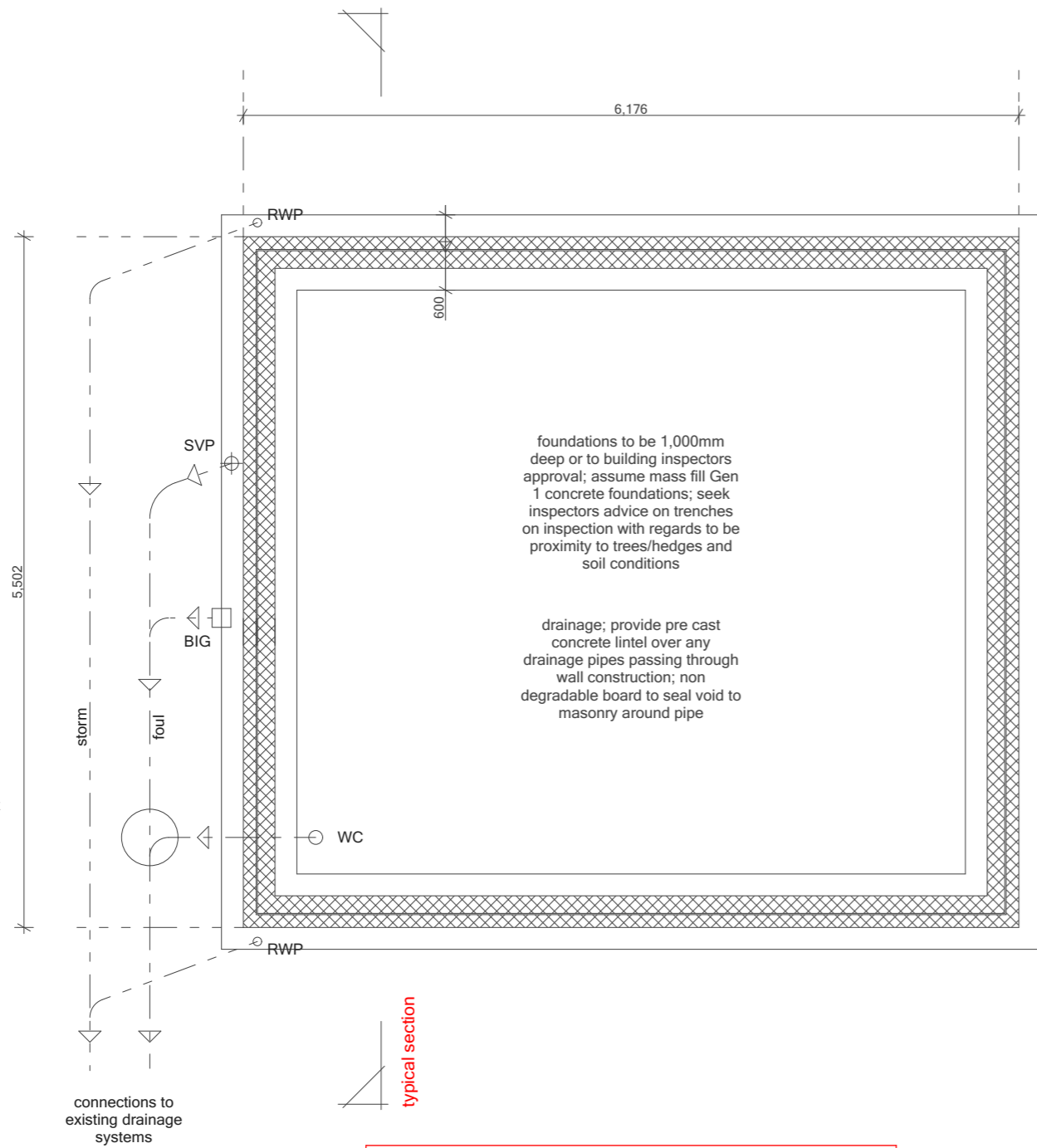
FOUNDATION PLAN
