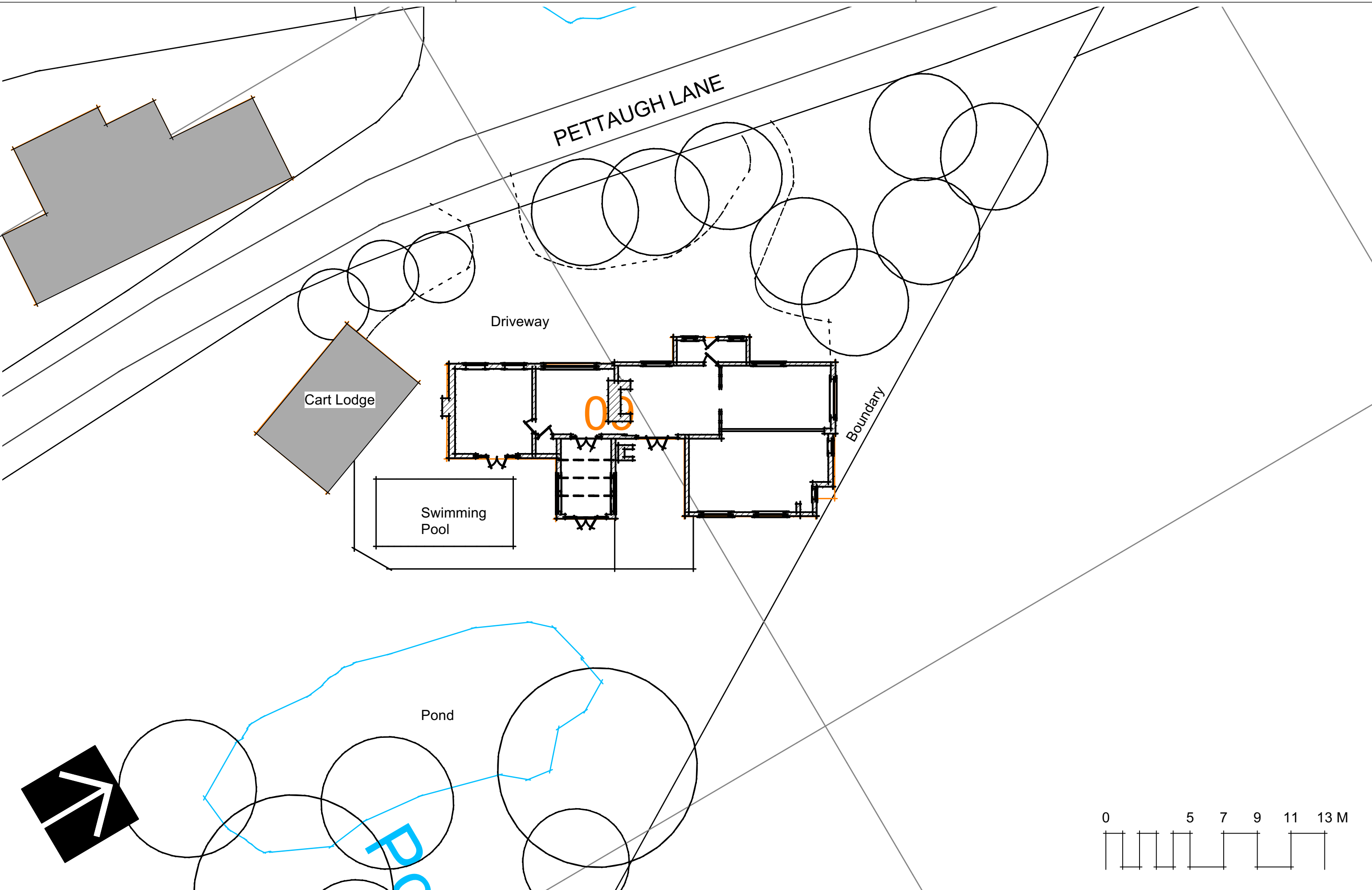
2 Block Plan-Existing Scale: 1:200
