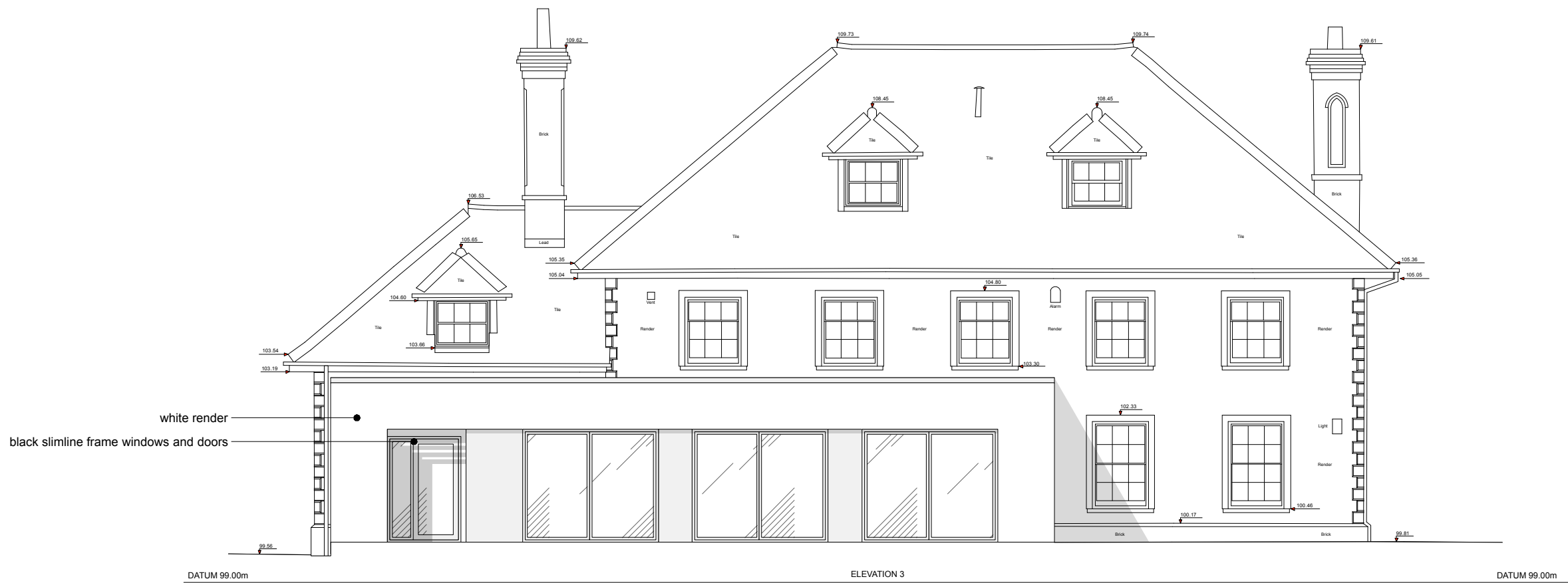
01 proposed north-east [rear] elevation Scale: 1:100
