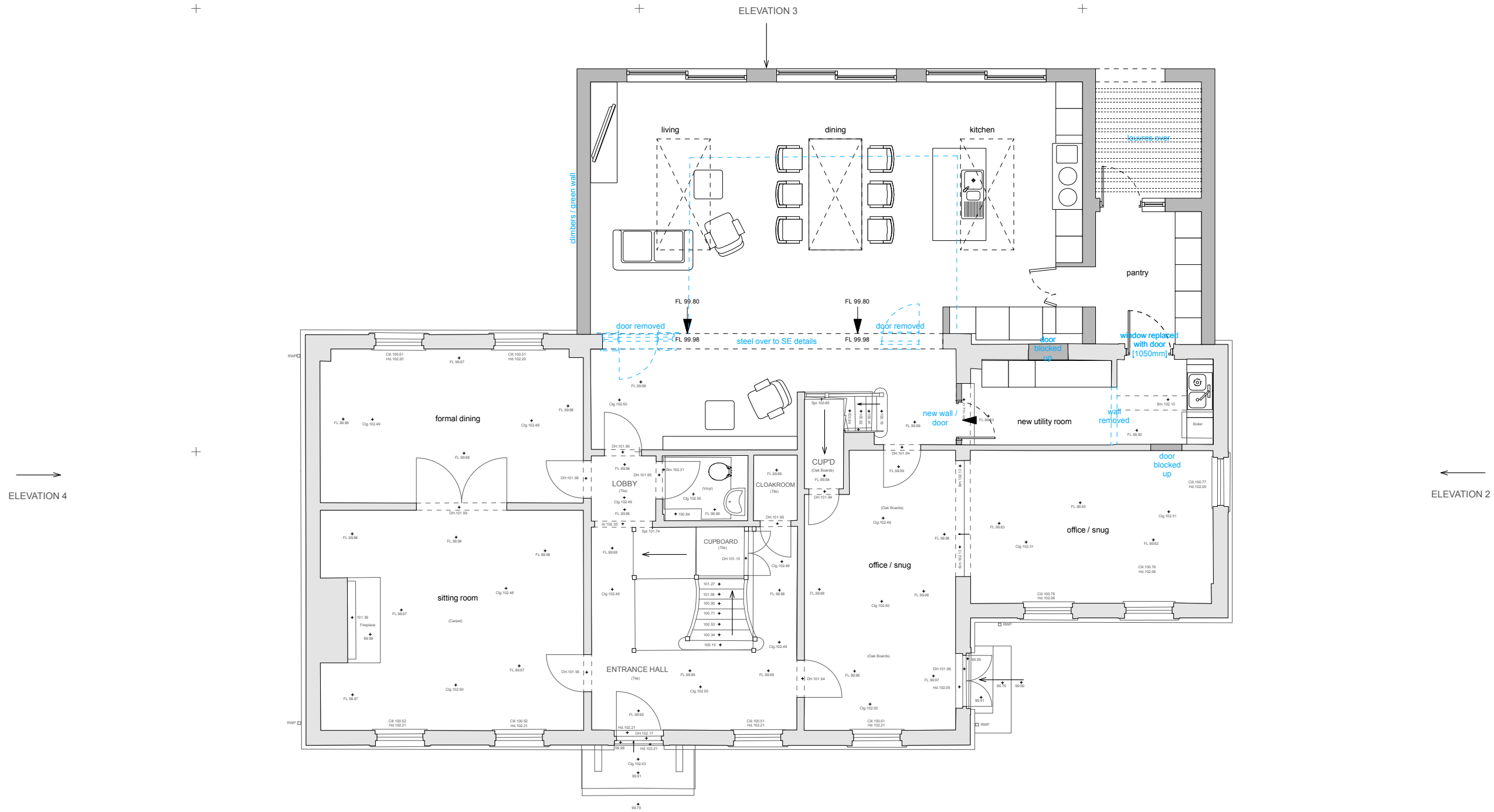
01 proposed ground floor plan Scale: 1:100
