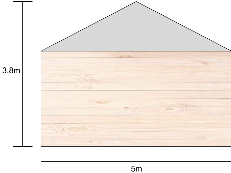
East Side Elevation
