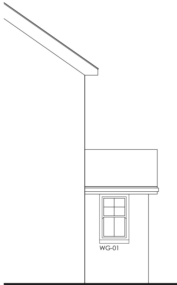
1 Proposed West Elevation 1 : 50
