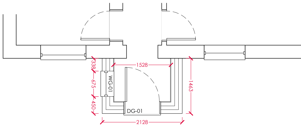
1 Proposed Ground Floor Plan 1 : 50
