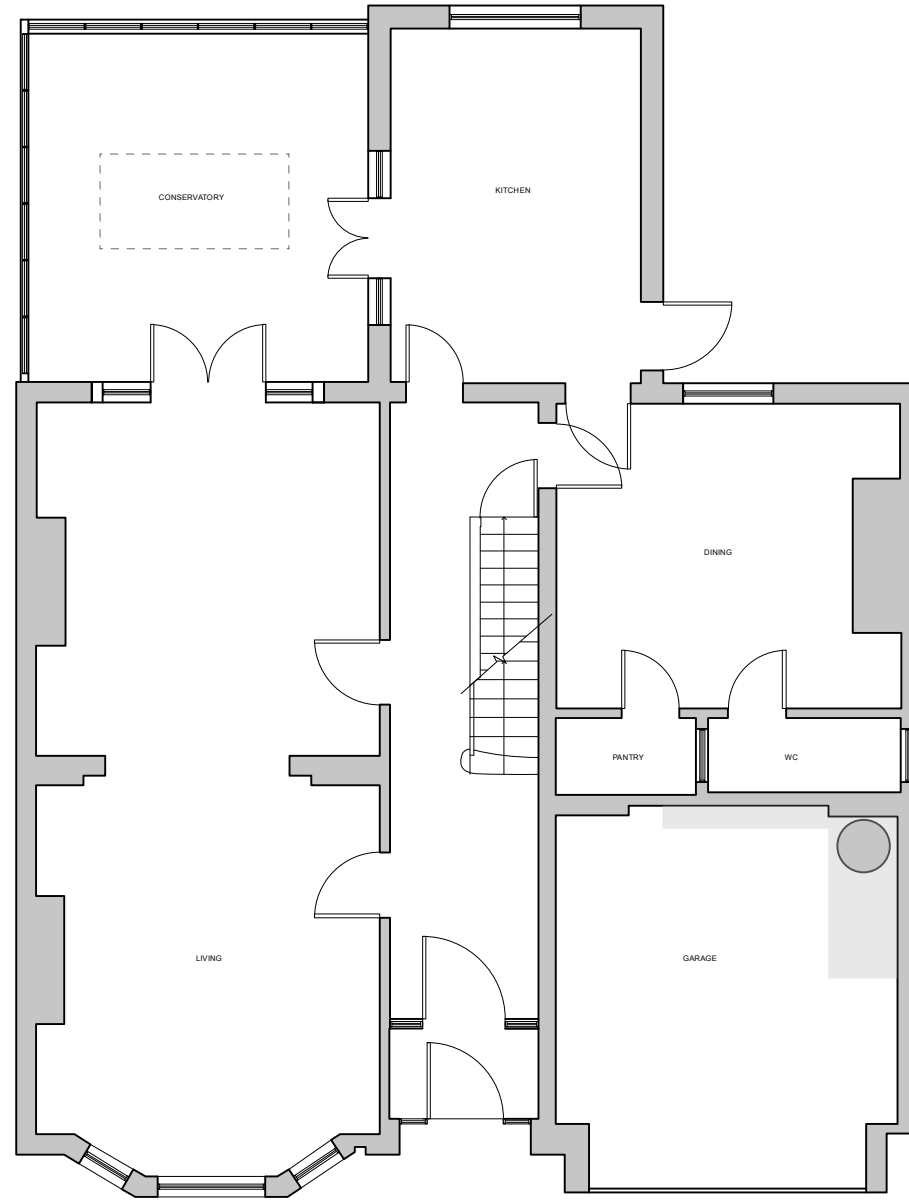
1 Ground Floor Scale: 1:100
