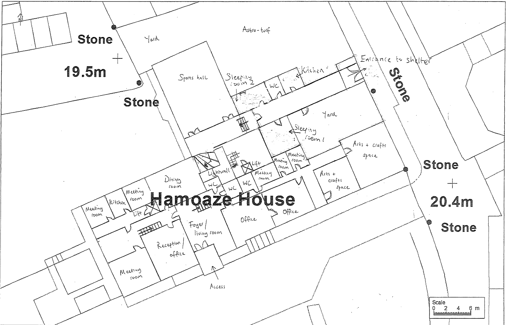
Existing Floor Plan 1:200 - Ground Floor
