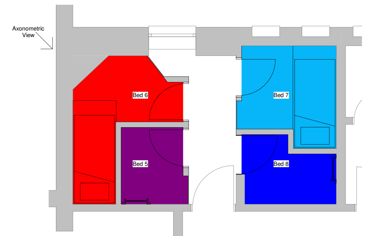
Room 2 Bottom Bunks (Cut 1000mm above Ground Floor Level) 1 : 50
