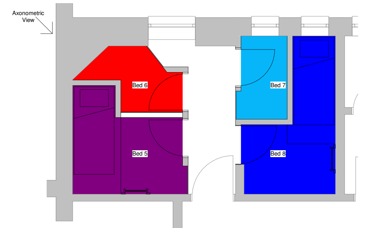
Room 2 Top Bunks (Cut 2000mm above Ground Floor Level) 1 : 50
