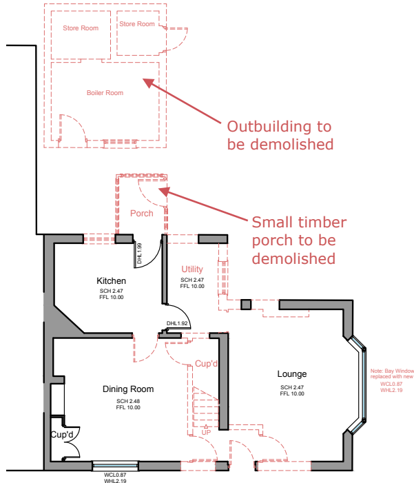
(Above) Ground Floor Demolition Plan Not to Scale
