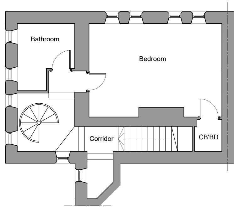
PROPOSED FIRST FLOOR LAYOUT
