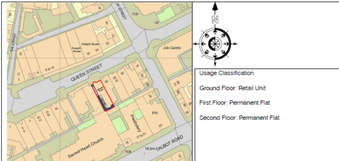
LOCATION PLAN 1:1250
